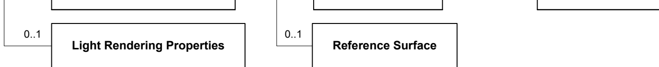
Figure 6.346—DRM_Union_Of_Geometry_Hierarchy
