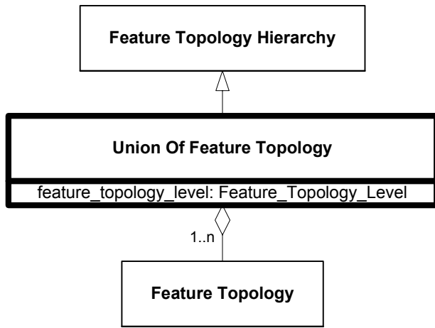
Figure 6.343—DRM_Union_Of_Feature_Topology
