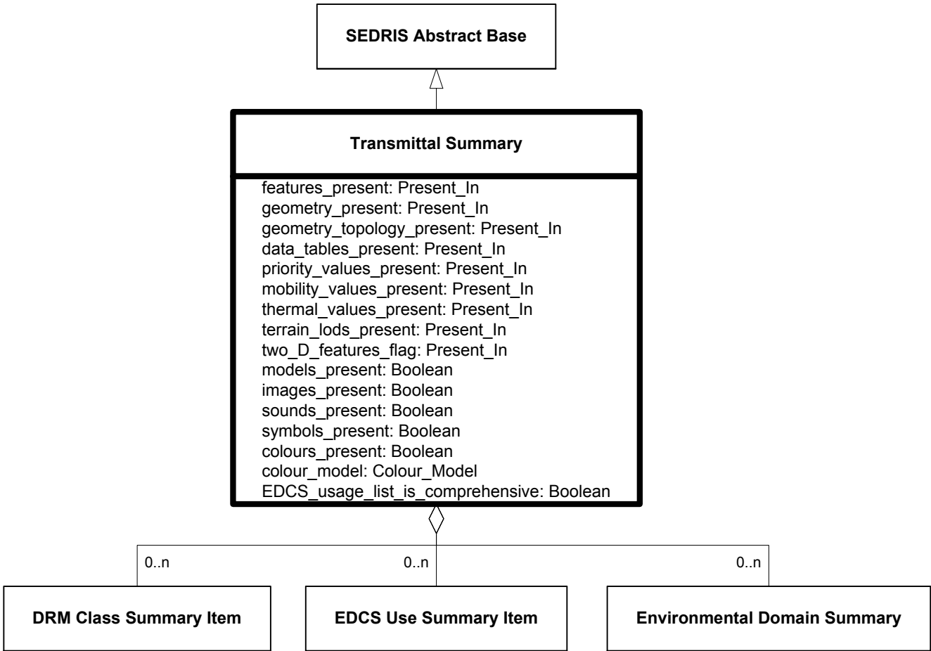
Figure 6.340 DRM_Transmittal_Summary
