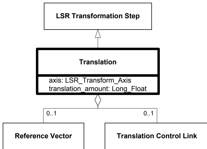
Figure 6.334—DRM_Translation
