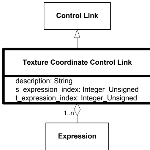
Figure 6.322—DRM_Texture_Coordinate_Control_Link
