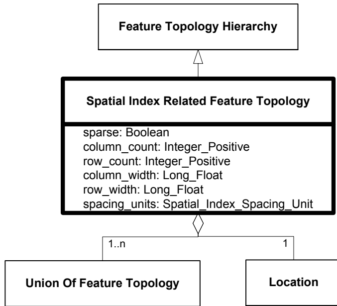
Figure 6.292—DRM_Spatial_Index_Related_Feature_Topology
