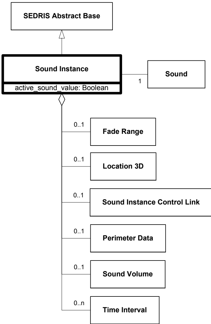
Figure 6.285—DRM_Sound_Instance
