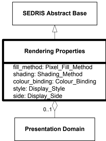
Figure 6.263—DRM_Rendering_Properties
