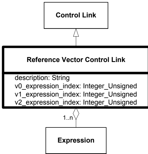
Figure 6.257—DRM_Reference_Vector_Control_Link
