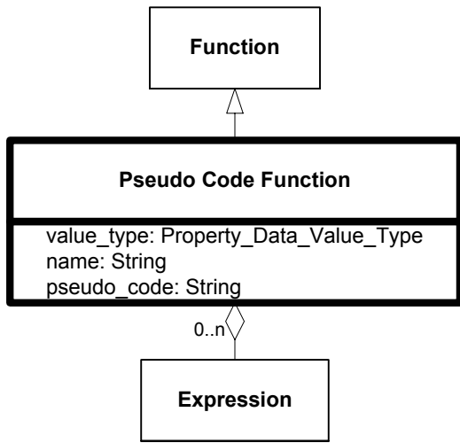
Figure 6.241—DRM_Pseudo_Code_Function
