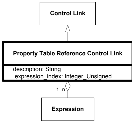
Figure 6.232—DRM_Property_Table_Reference_Control_Link
