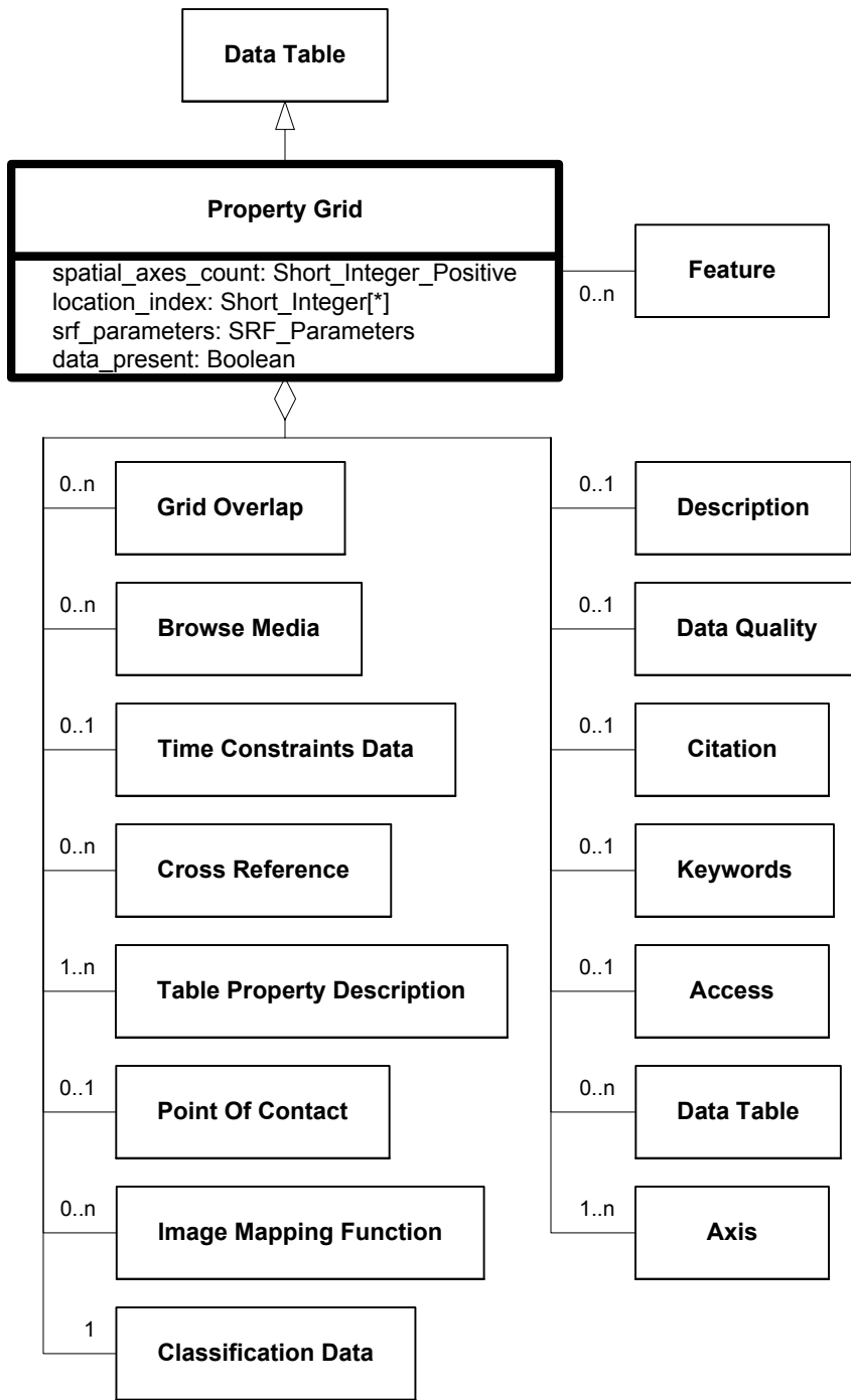
Figure 6.221—DRM_Property_Grid
