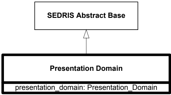
Figure 6.208—DRM_Presentation_Domain
