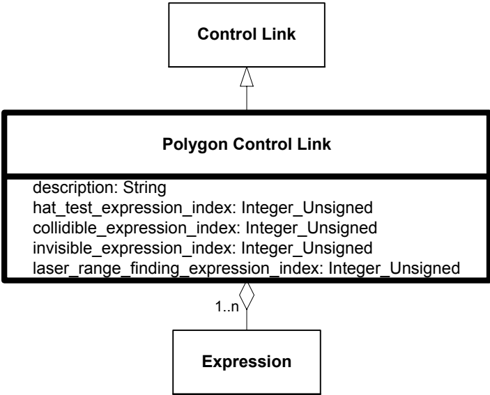
Figure 6.204—DRM_Polygon_Control_Link
