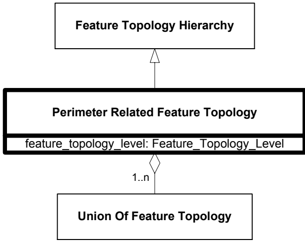
Figure 6.196—DRM_Perimeter_Related_Feature_Topology
