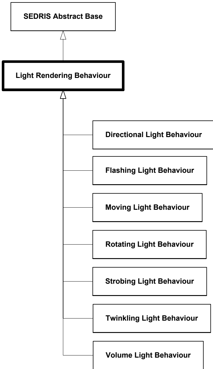
Figure 6.152—DRM_Light_Rendering_Behaviour
