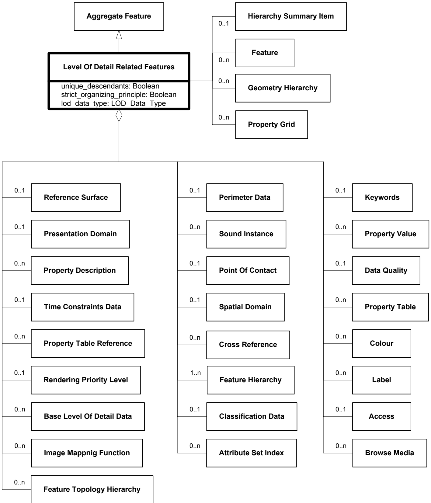
Figure 6.147—DRM_Level_Of_Detail_Related_Features
