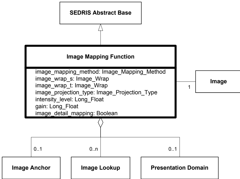
Figure 6.135—DRM_Image_Mapping_Function
