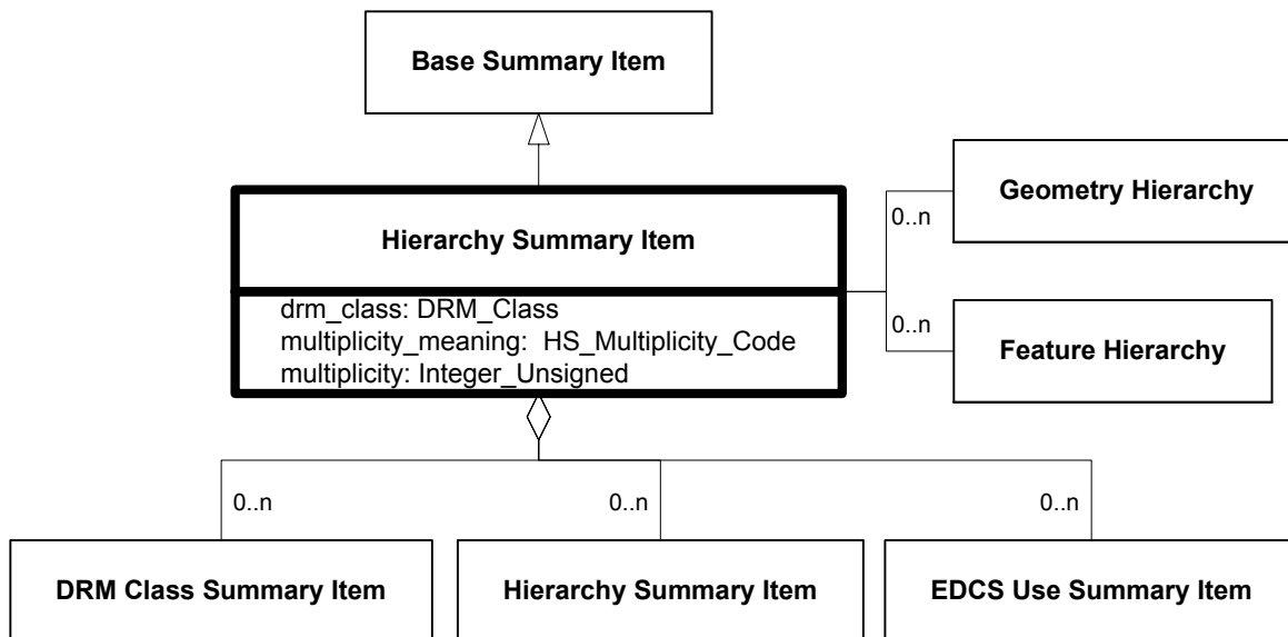
Figure 6.123—DRM_Hierarchy_Summary_Item
