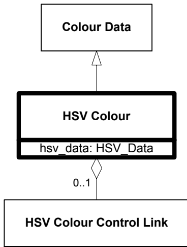
Figure 6.126—DRM_HSV_Colour
