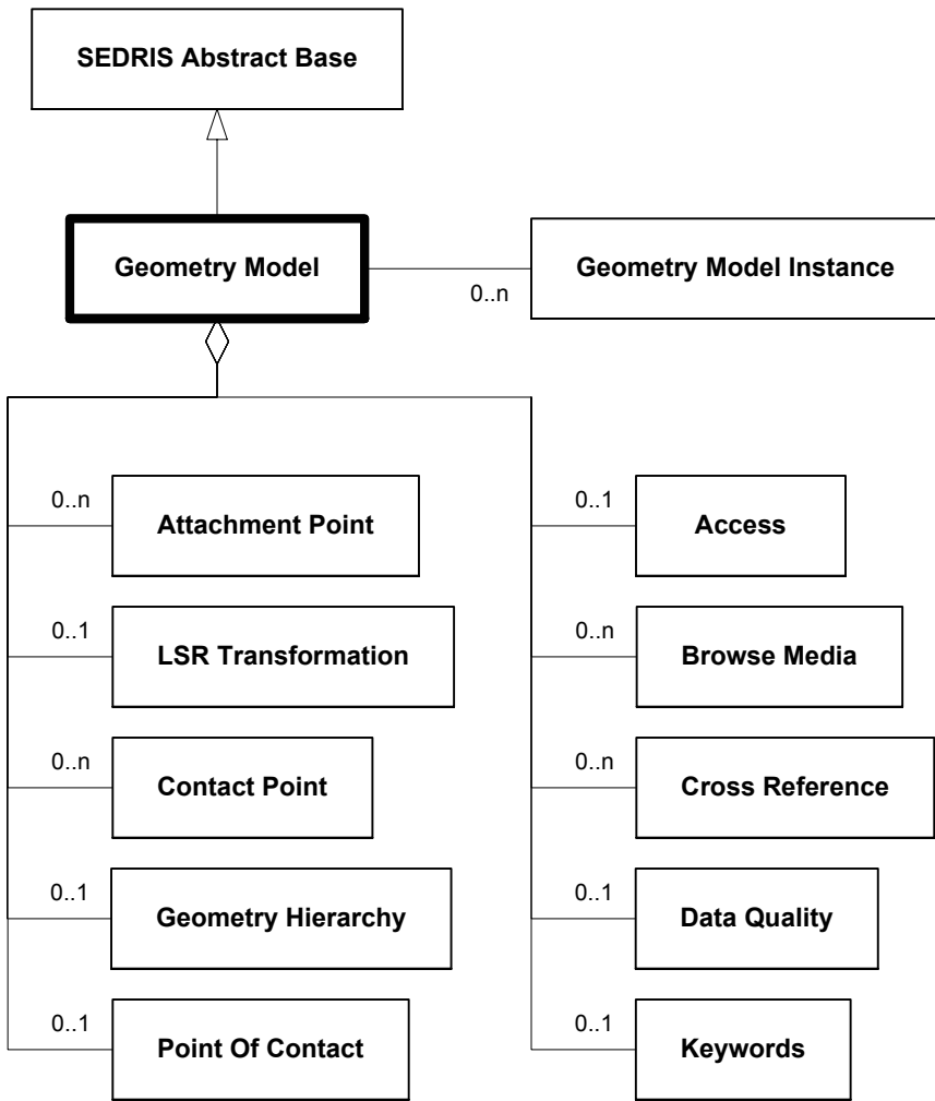
Figure 6.112—DRM_Geometry_Model
