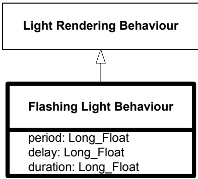
Figure 6.102—DRM_Flashing_Light_Behaviour
