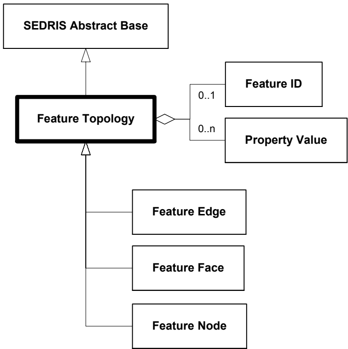
Figure 6.96—DRM_Feature_Topology
