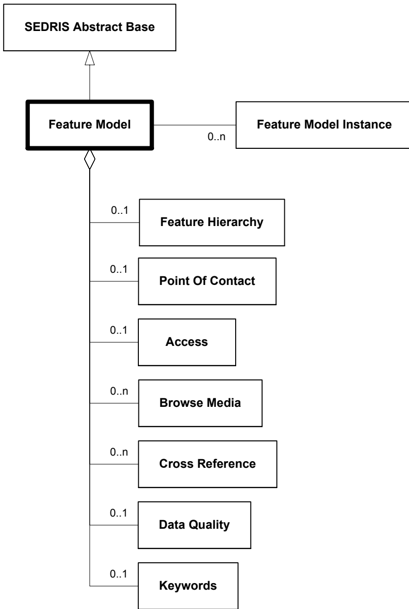
Figure 6.93—DRM_Feature_Model
