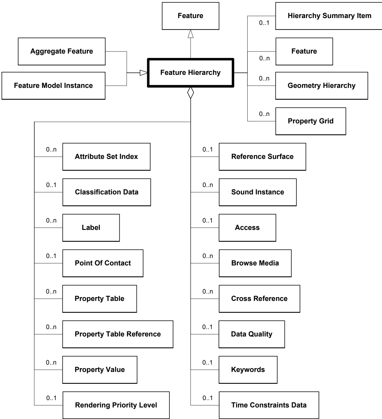
Figure 6.92—DRM_Feature_Hierarchy
