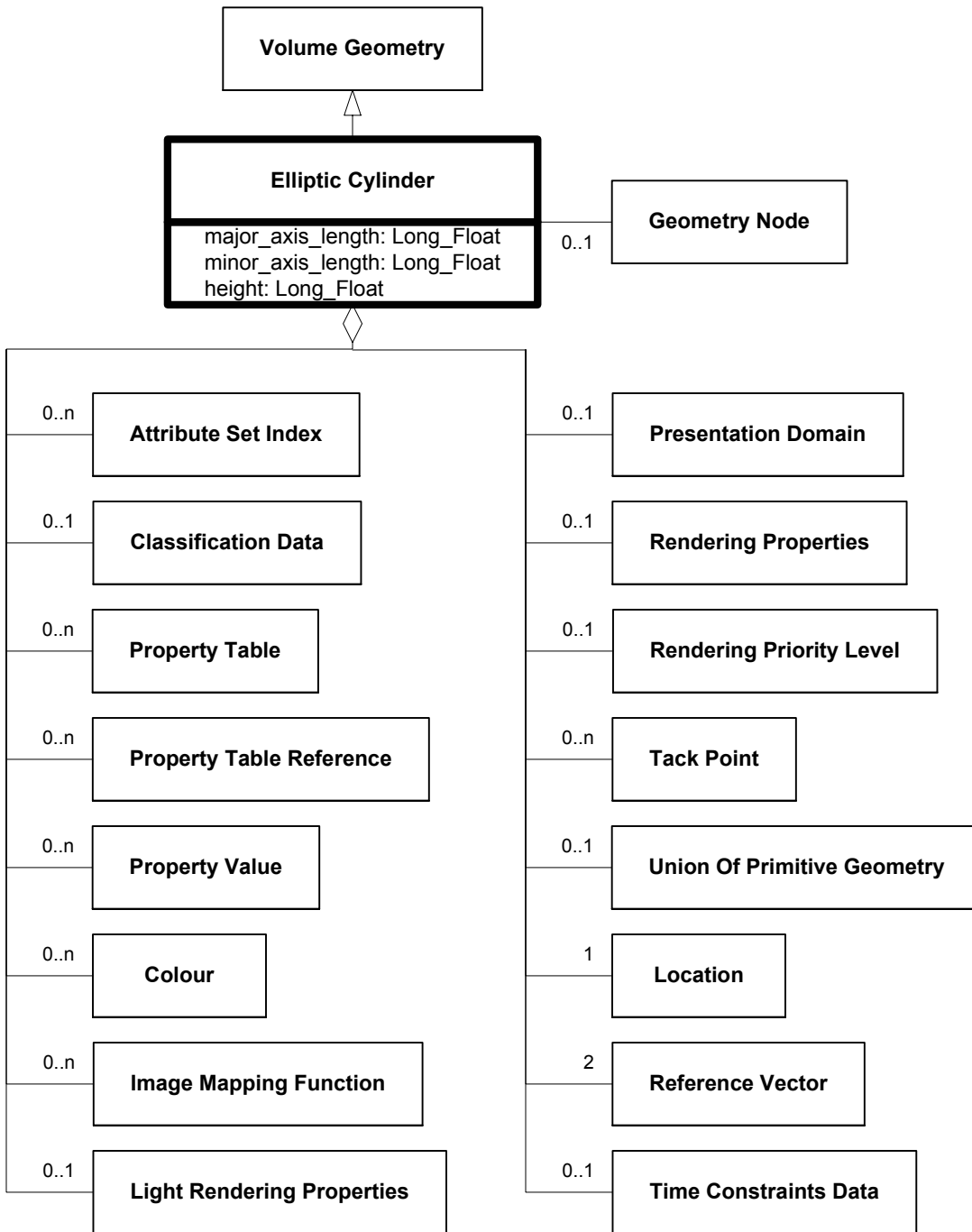
Figure 6.79—DRM_Elliptic_Cylinder
