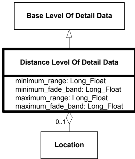
Figure 6.67—DRM_Distance_Level_Of_Detail_Data
