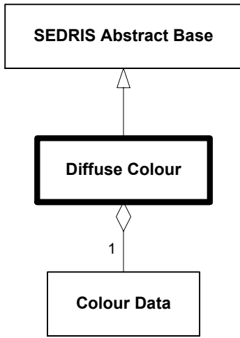
Figure 6.65—DRM_Diffuse_Colour
