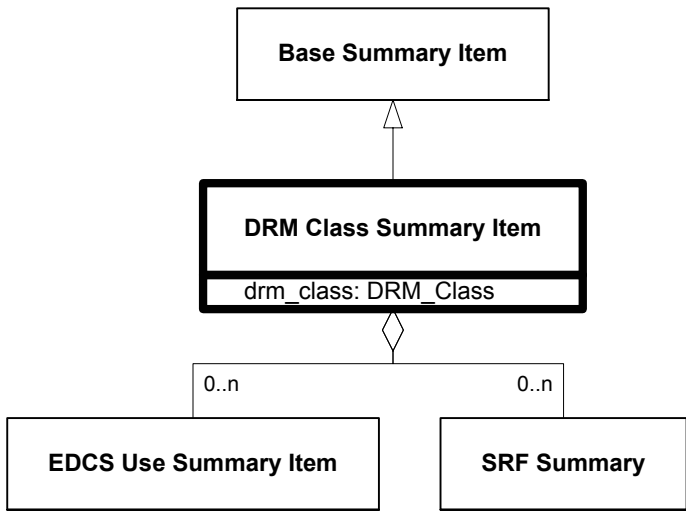
Figure 6.68—DRM_Class_Summary_Item
