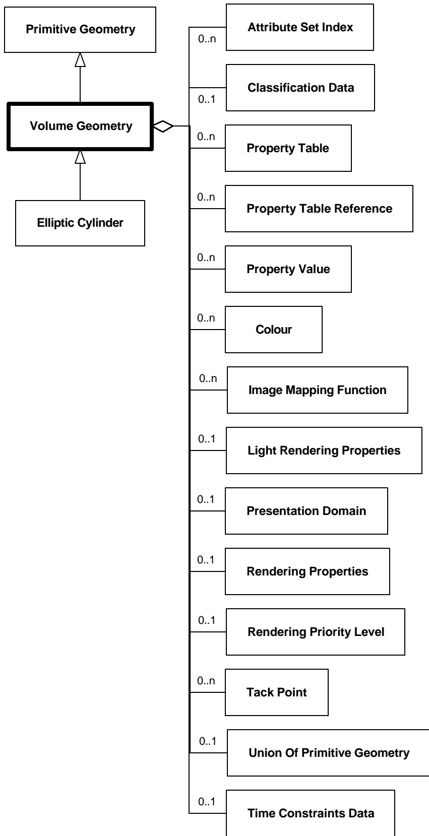
Diagram 6.321--DRM_Volume_Geometry
