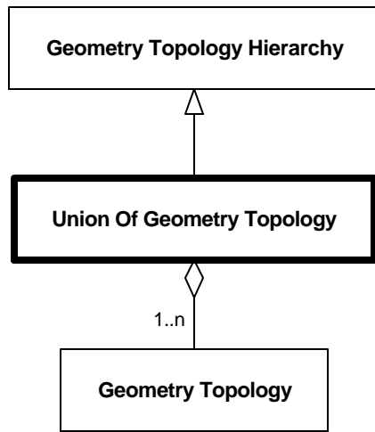
Diagram 6.311--DRM_Union_Of_Geometry_Topology
