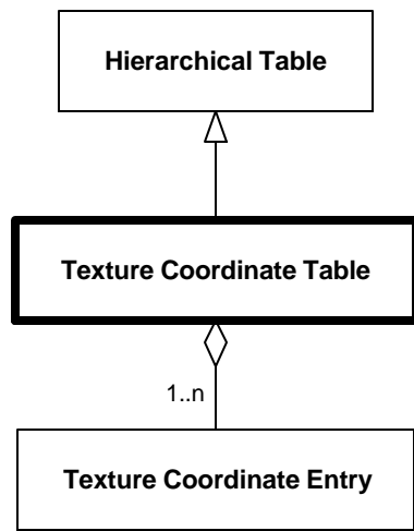
Diagram 6.291--DRM_Texture_Coordinate_Table
