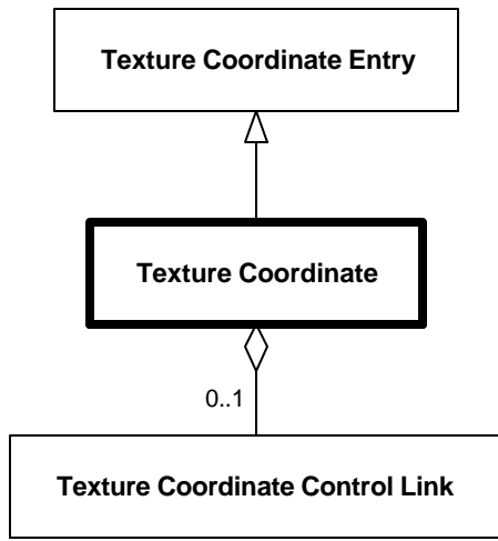
Diagram 6.287--DRM_Texture_Coordinate
