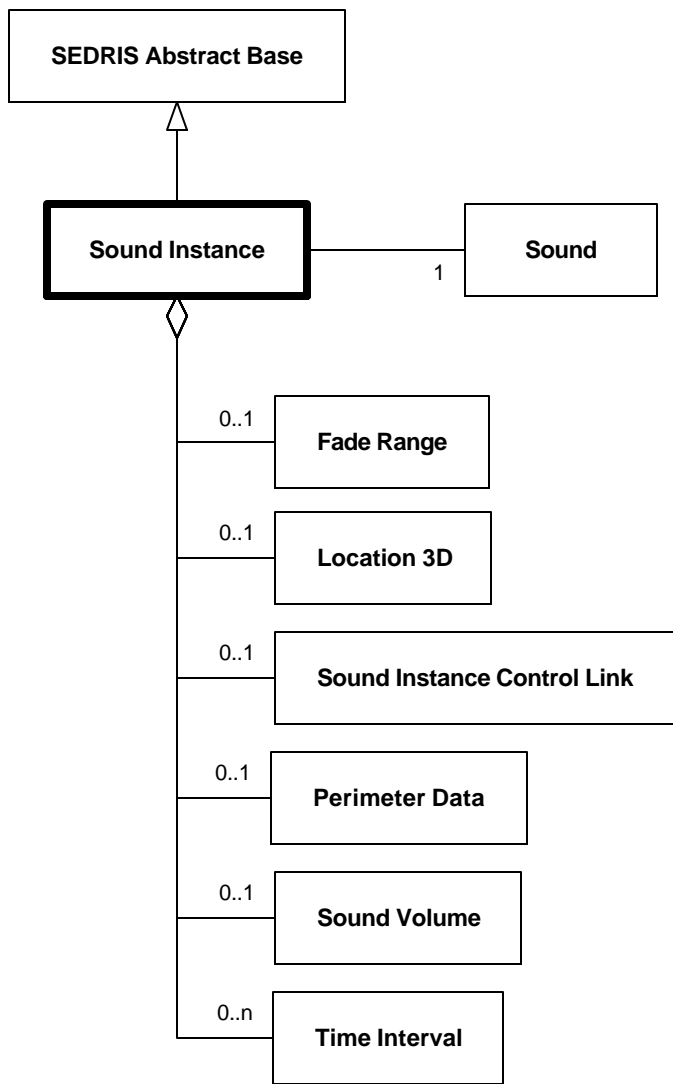
Diagram 6.259--DRM_Sound_Instance
