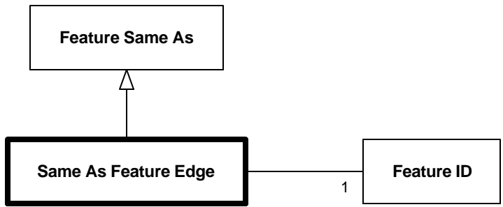
Diagram 6.243--DRM_Same_As_Feature_Edge
