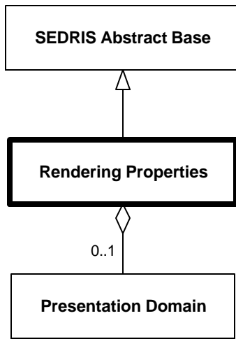
Diagram 6.237--DRM_Rendering_Properties
