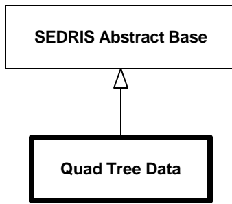
Diagram 6.223--DRM_Quad_Tree_Data
