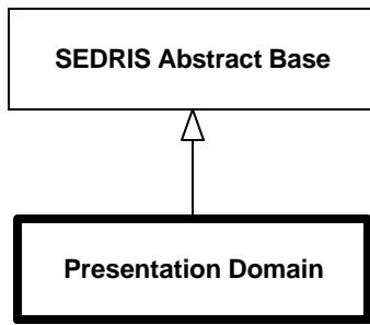
Diagram 6.202--DRM_Presentation_Domain
