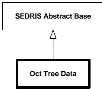
Diagram 6.183--DRM_Oct_Tree_Data
