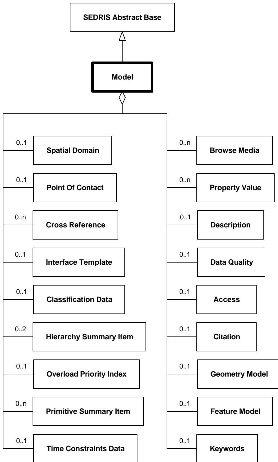
Diagram 6.178—DRM_Model
