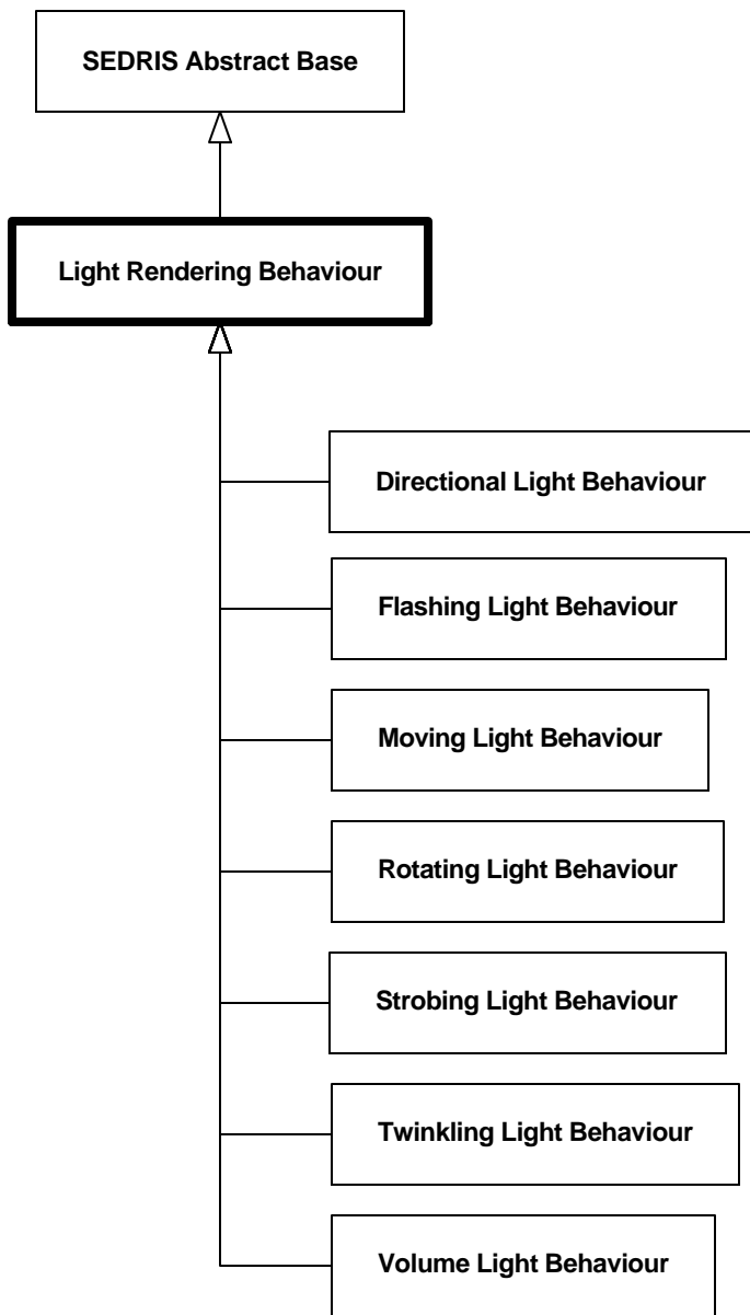
Diagram 6.153—DRM_Light_Rendering_Behaviour
