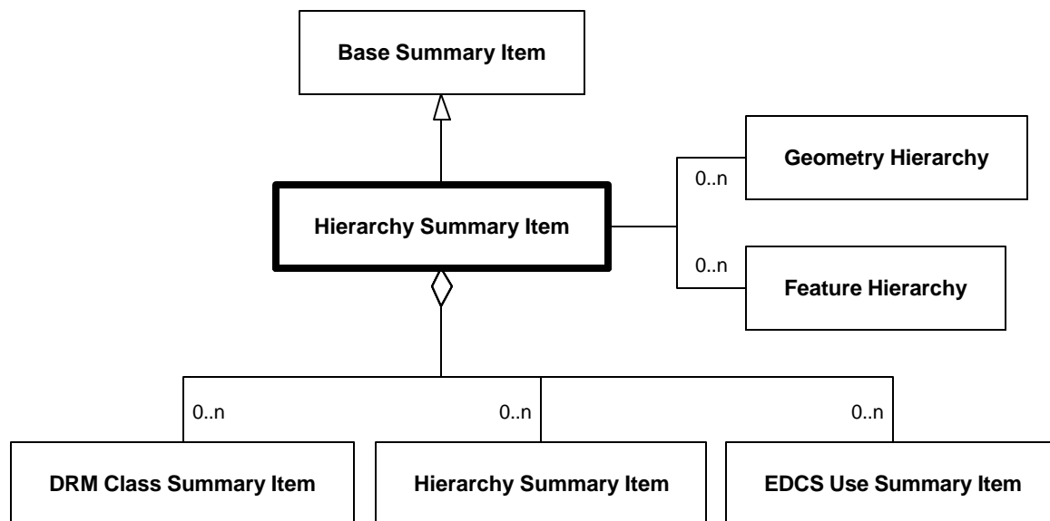
Diagram 6.130—DRM_Hierarchy_Summary_Item
