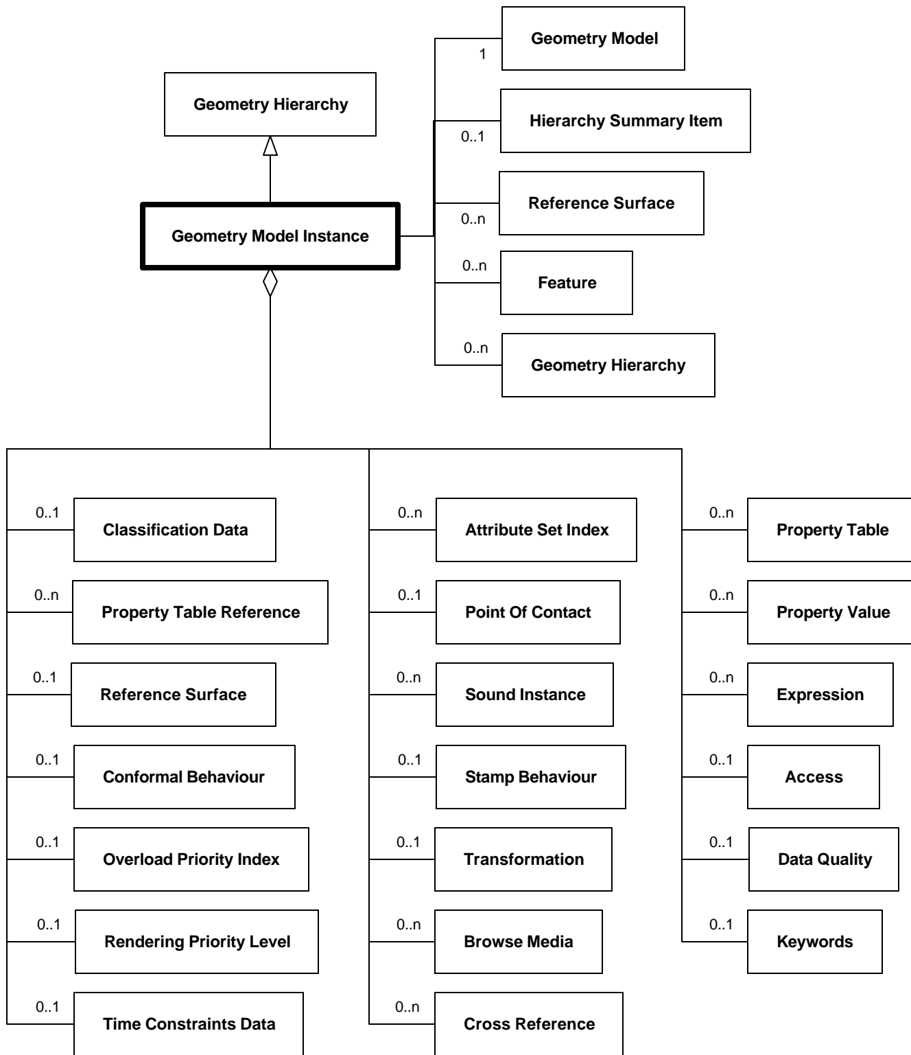
Diagram 6.119—DRM_Geometry_Model_Instance
