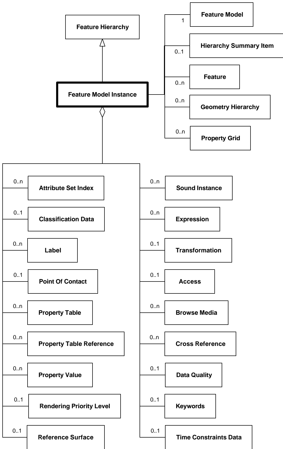
Diagram 6.98—DRM_Feature_Model_Instance
