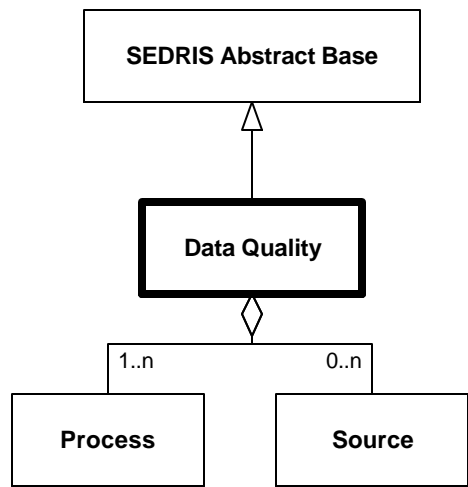
Diagram 6.69—DRM_Data_Quality
