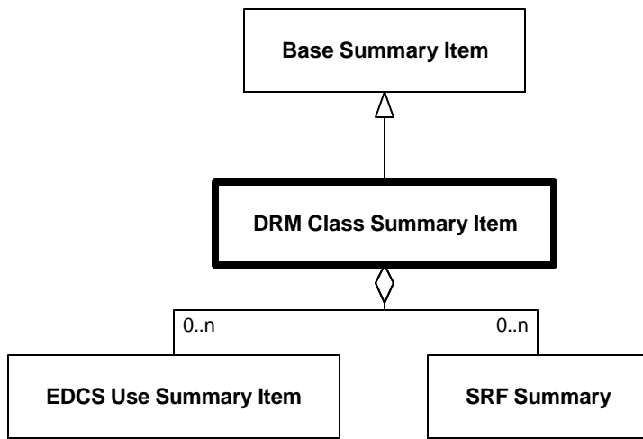
Diagram 6.76—DRM_Class_Summary_Item
