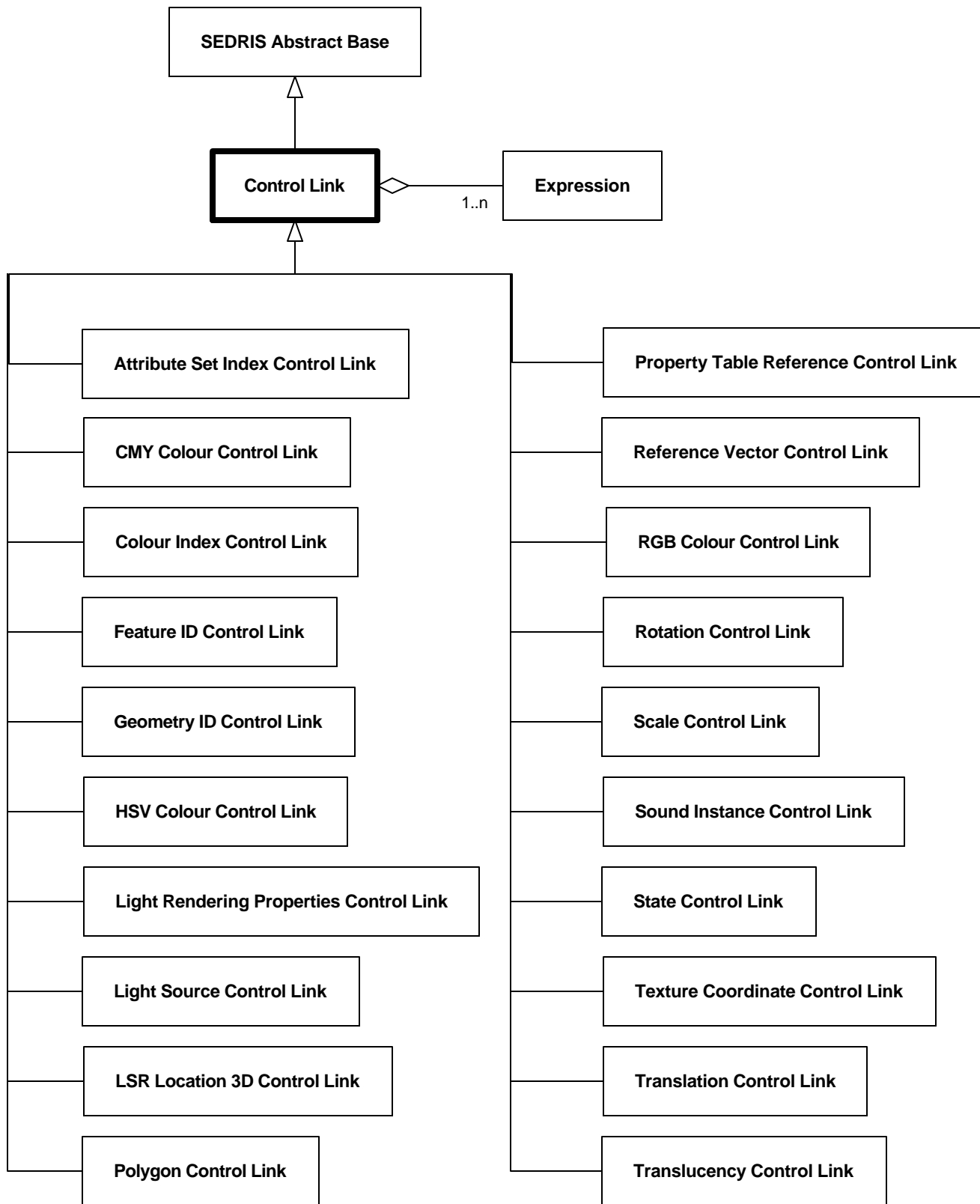
Diagram 6.66--DRM_Control_Link
