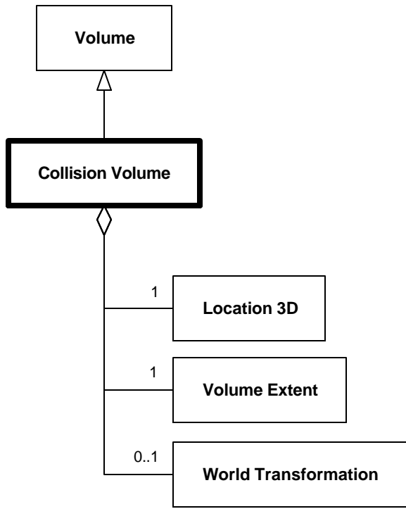
Diagram 6.48--DRM_Collision_Volume
