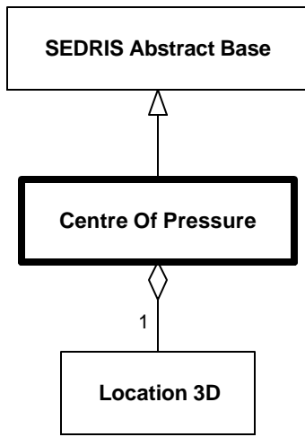
Diagram 6.41--DRM_Centre_Of_Pressure
