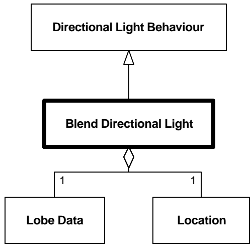
Diagram 6.35--DRM_Blend_Directional_Light
